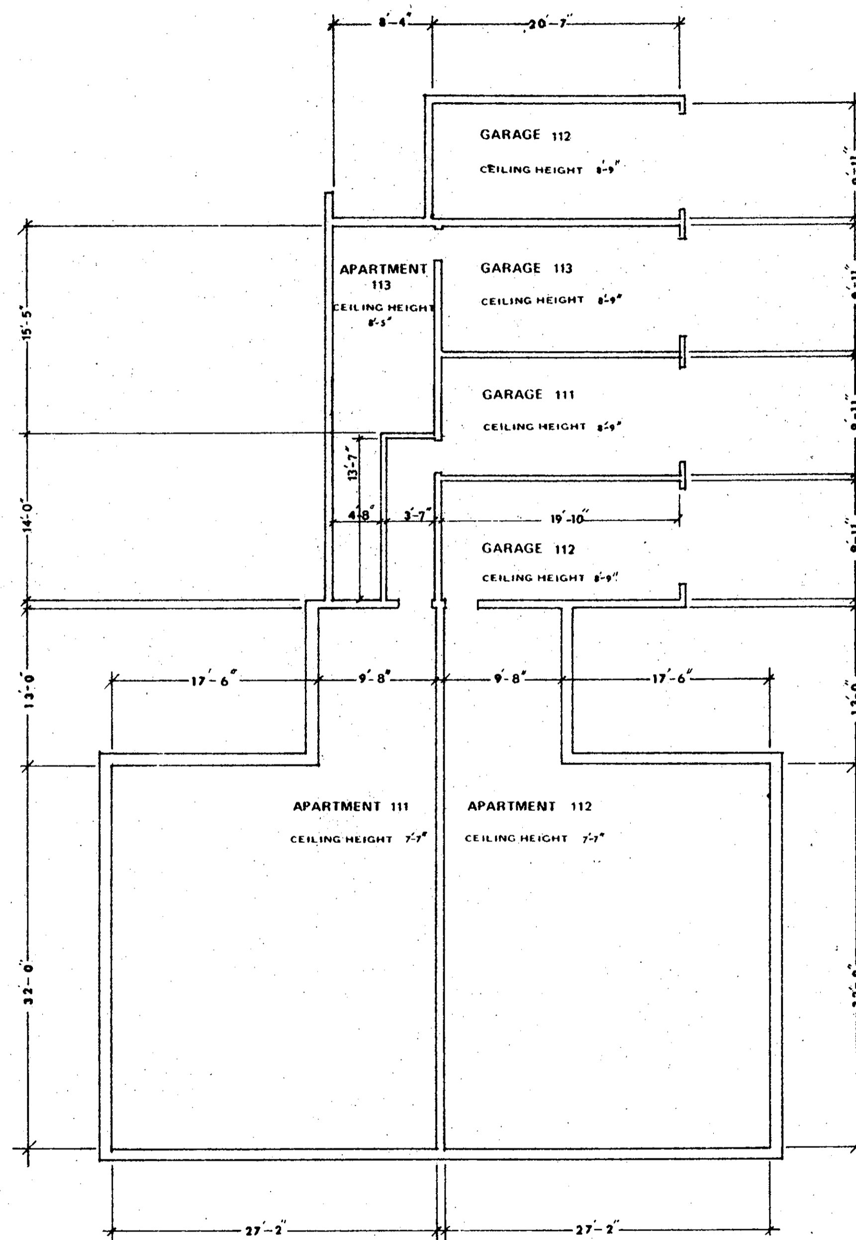
BASEMENT
