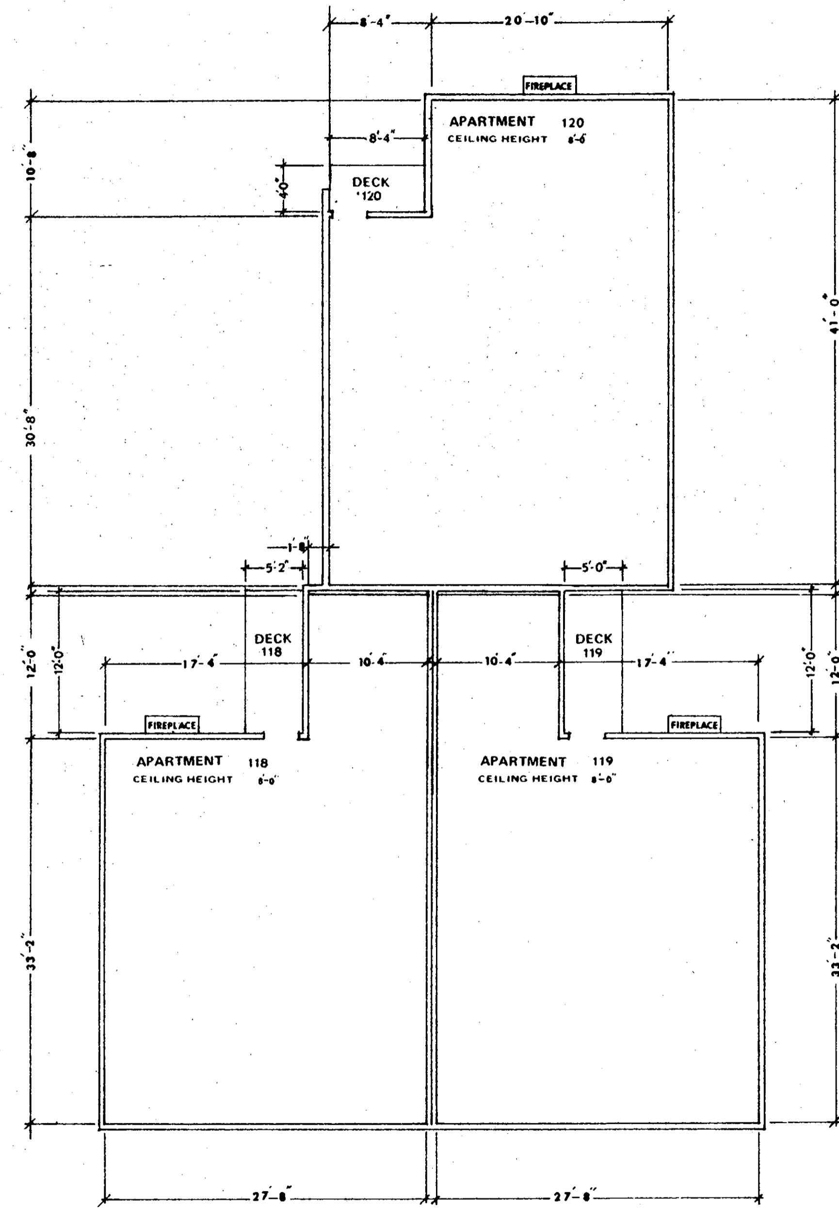
FIRST FLOOR
