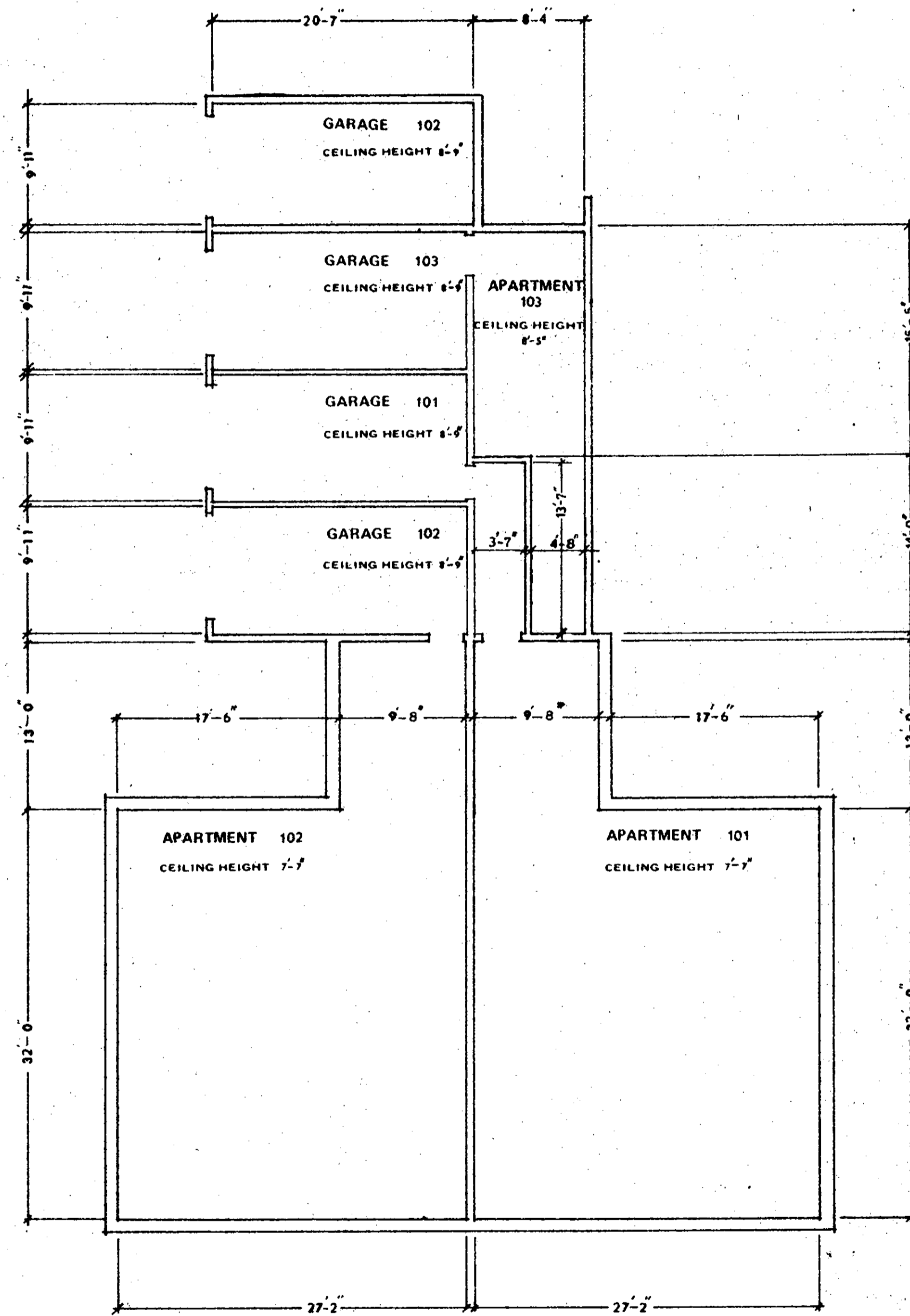
BASEMENT
