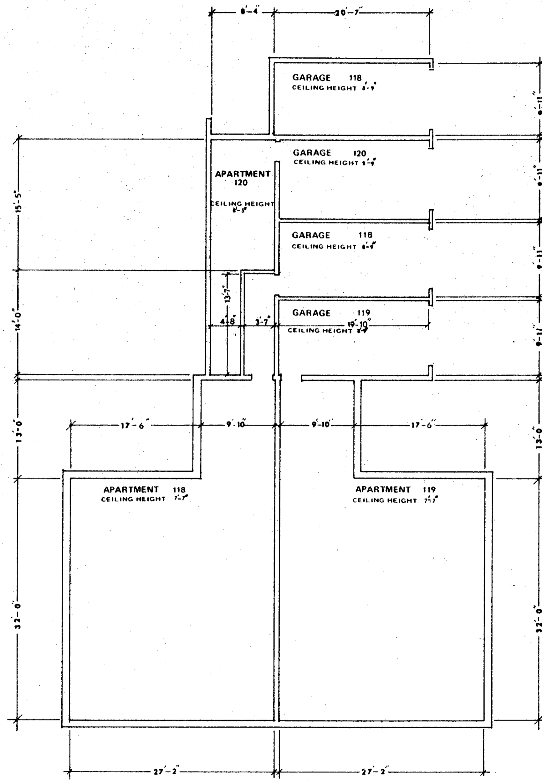
BASEMENT
