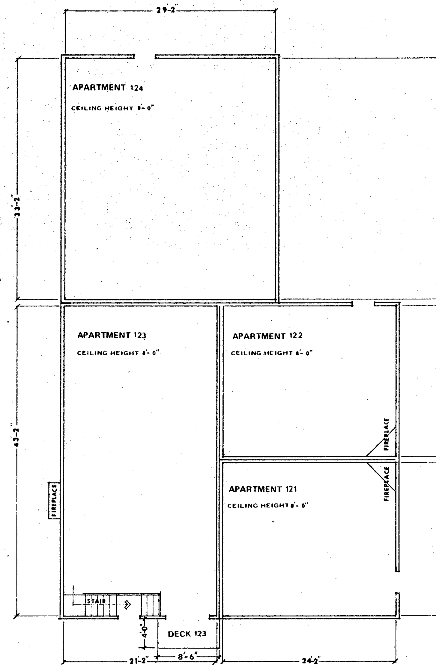
FIRST FLOOR
