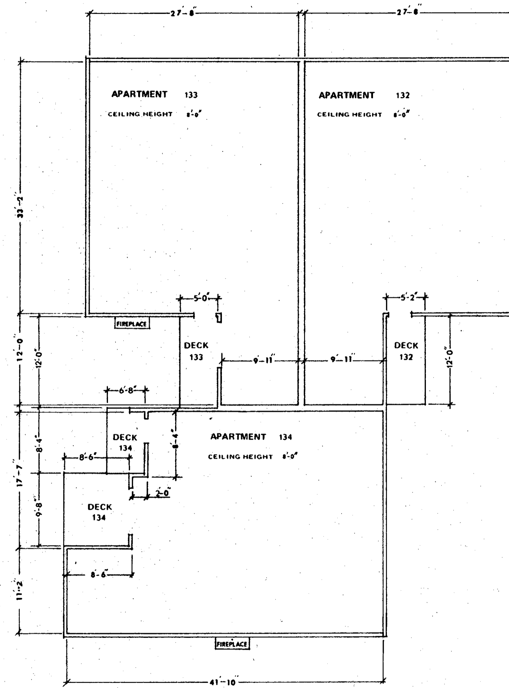
FIRST FLOOR
