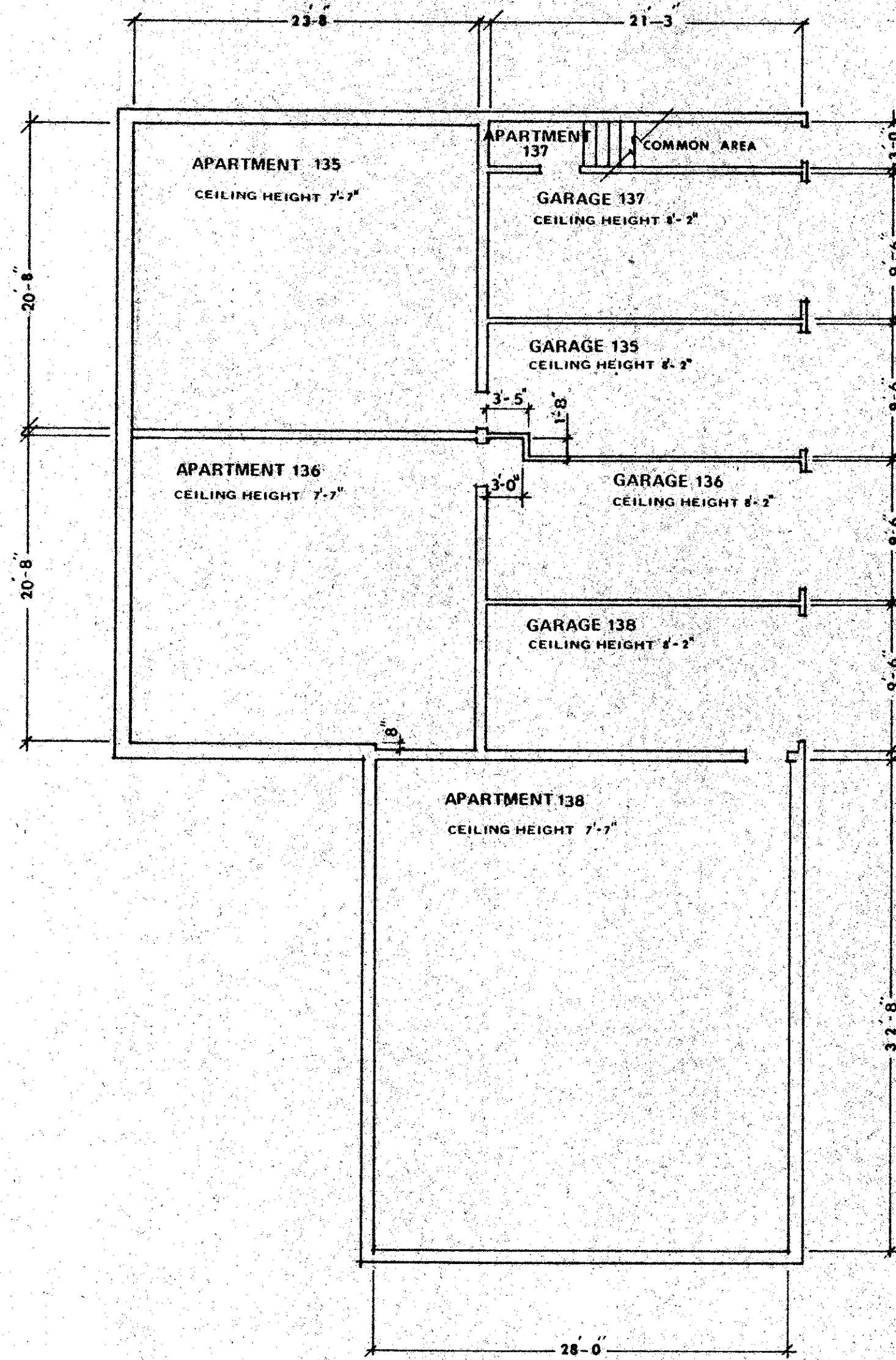
BASEMENT
