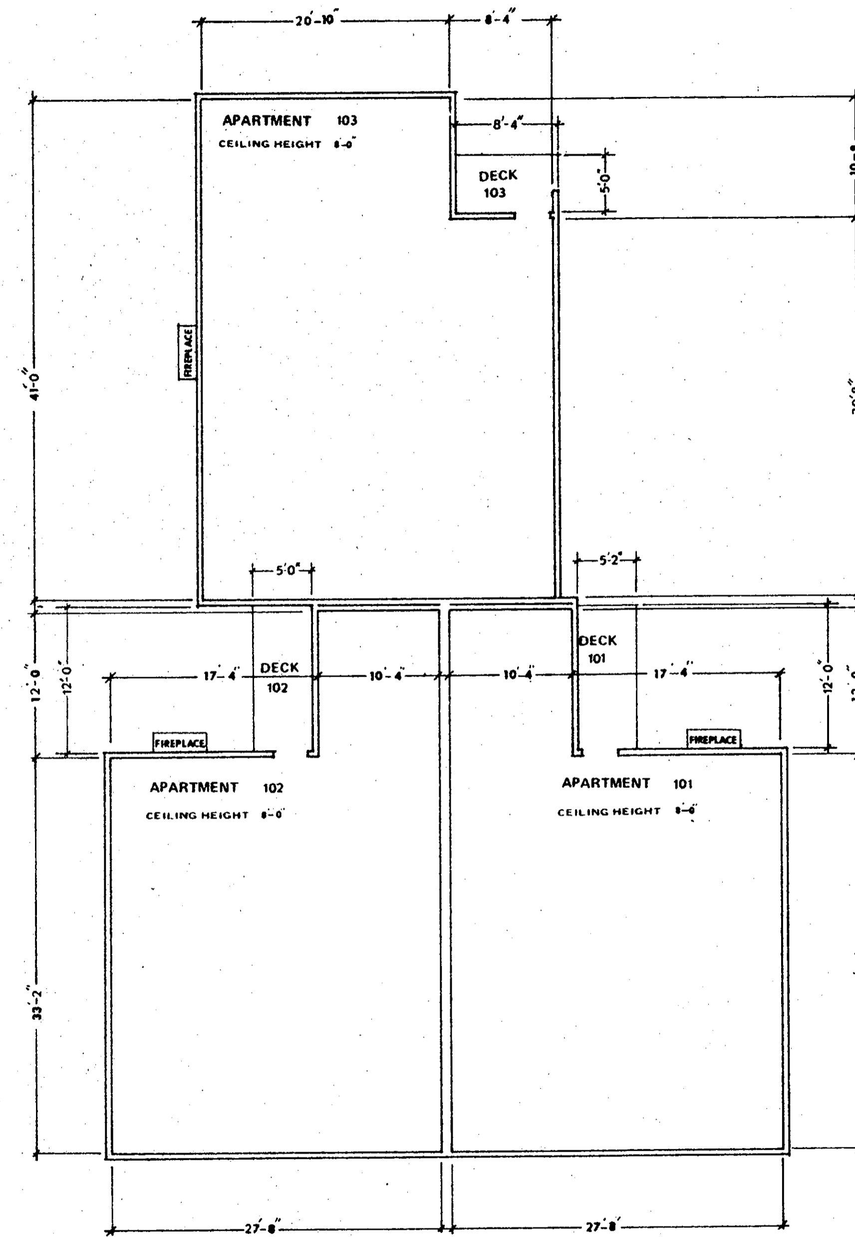
FIRST FLOOR
