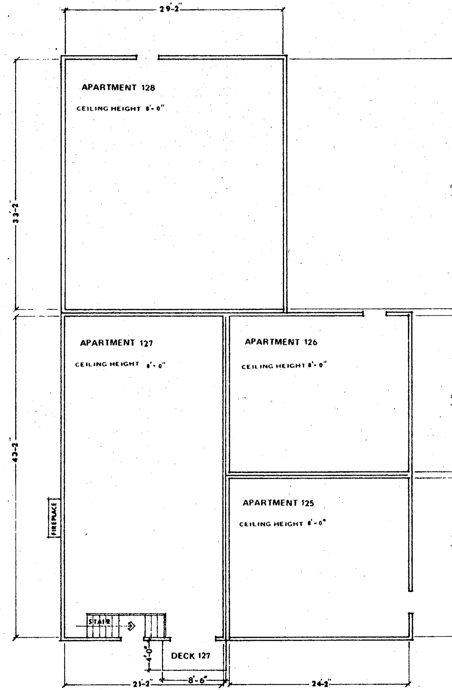
FIRST FLOOR
