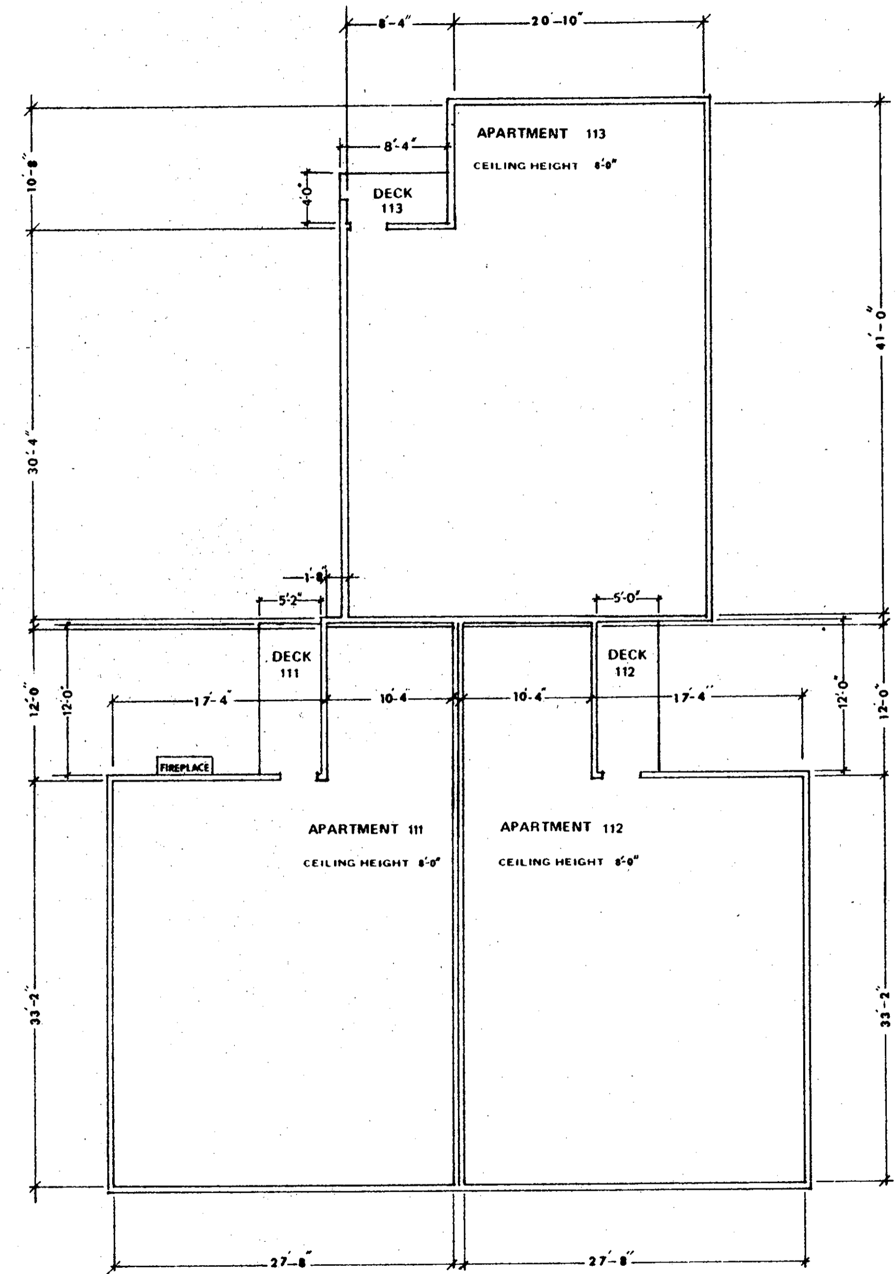
FIRST FLOOR
