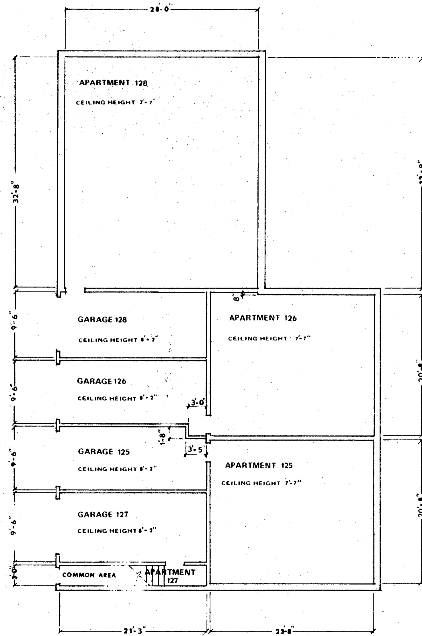
BASEMENT
