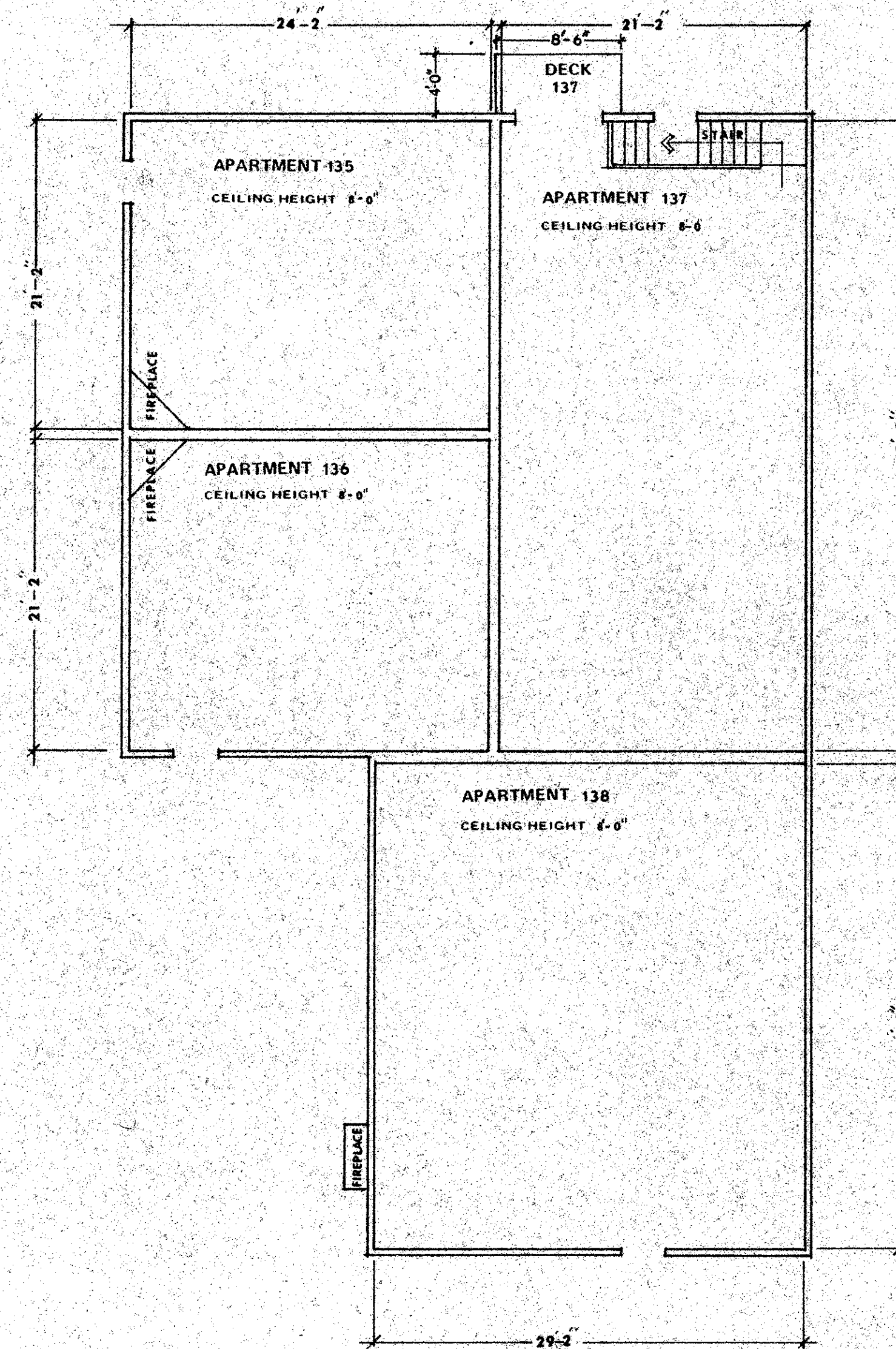
FIRST FLOOR
