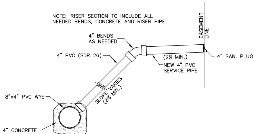
407 - SERVICE RISER DETAIL 407 - Serv Riser.dwg 6/2015
